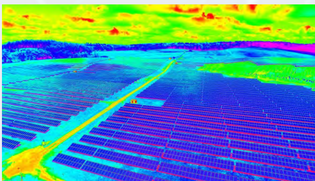
Infrared Drone Thermography
